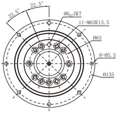
输出端/OUTPUT
