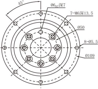
输出端/OUTPUT
