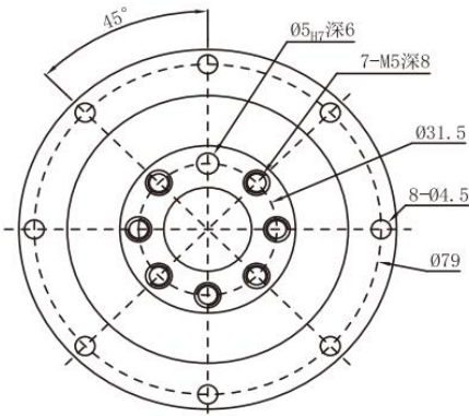
输出端/OUTPUT
